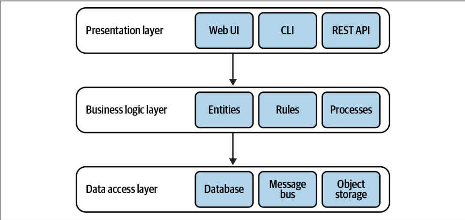
Figure 8-5. Layered architecture
