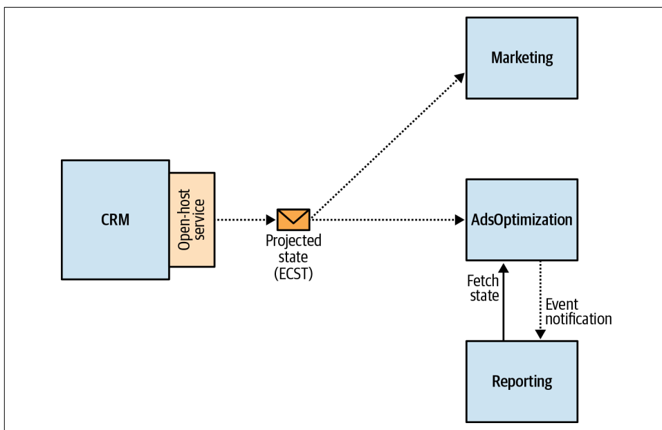
Figure 15-6. Refactored system
